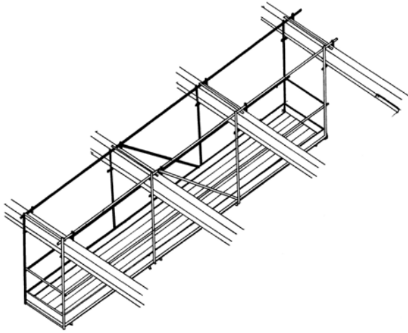
Hung scaffold
